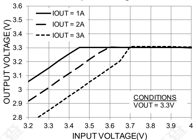
Dropout Voltage
