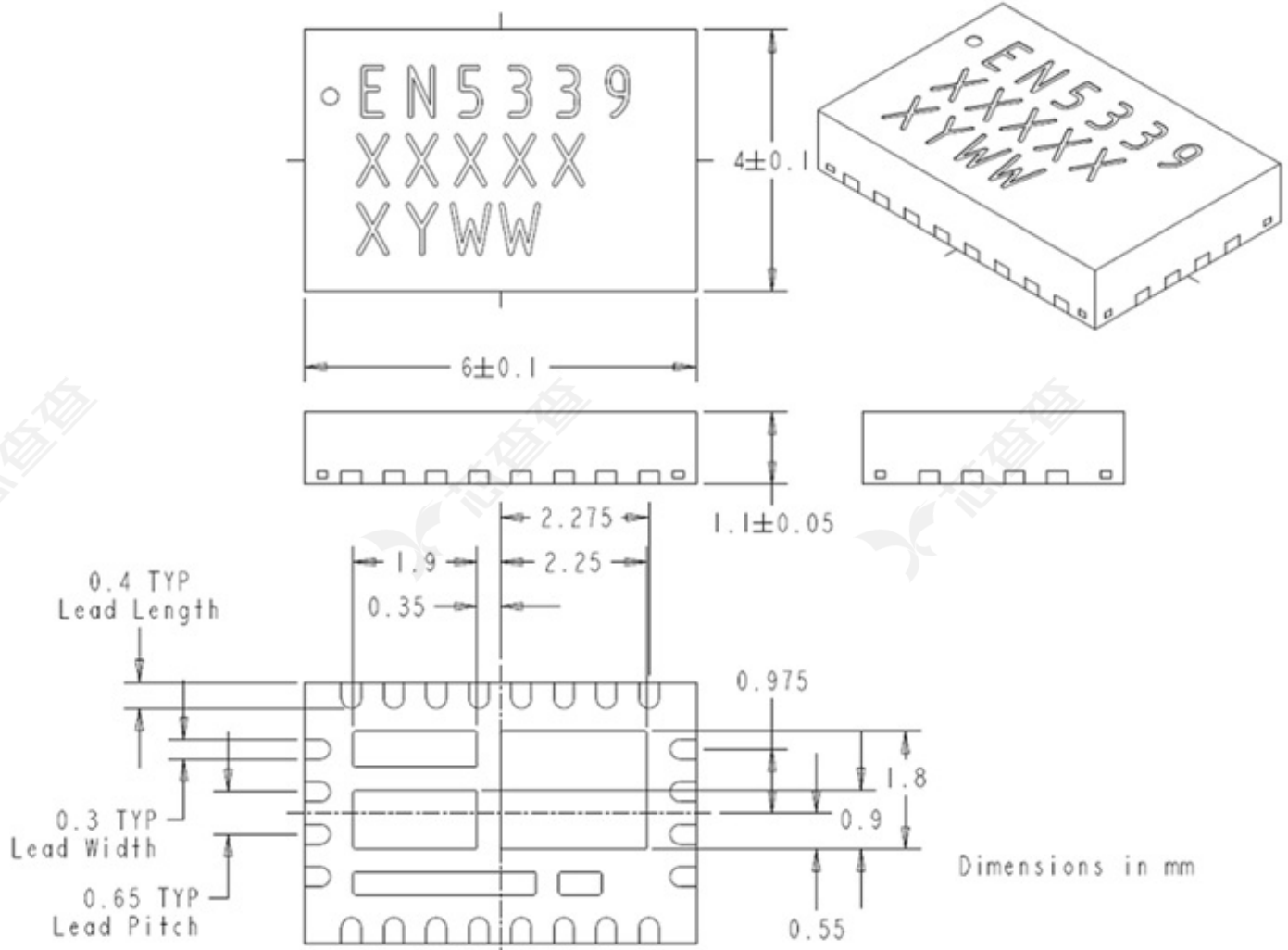
Figure 12: EN5339QI Package Dimensions (Bottom View)
